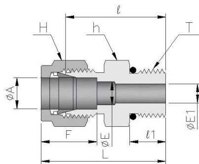
UNF straight thred
