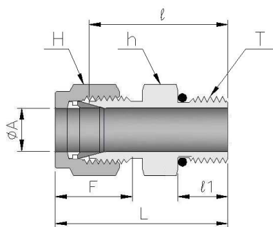
UNF stright thred
